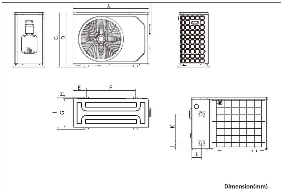
SUN Series 15 kW
